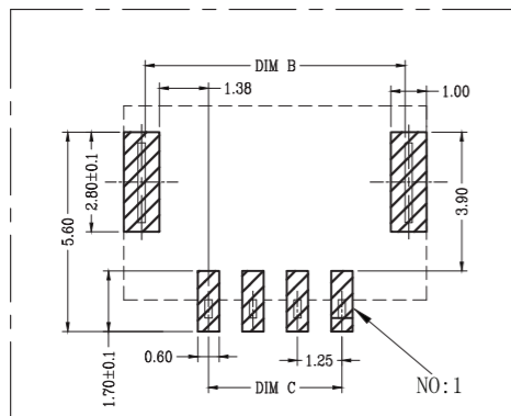
Recommended P.C.B Layout General Tolerance \pm 0.05
